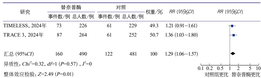
图6 在4.5~24 h时间窗内, 替奈普酶组与对照组急性缺血性卒中患者3个月极好功能结局 (mRS评分0~1分) RR Figure 6 RR for excellent functional outcome (mRS score 0-1) at 3 months in acute ischemic stroke patients in the tenecteplase and the control groups within the 4.5 to 24 hours time window
