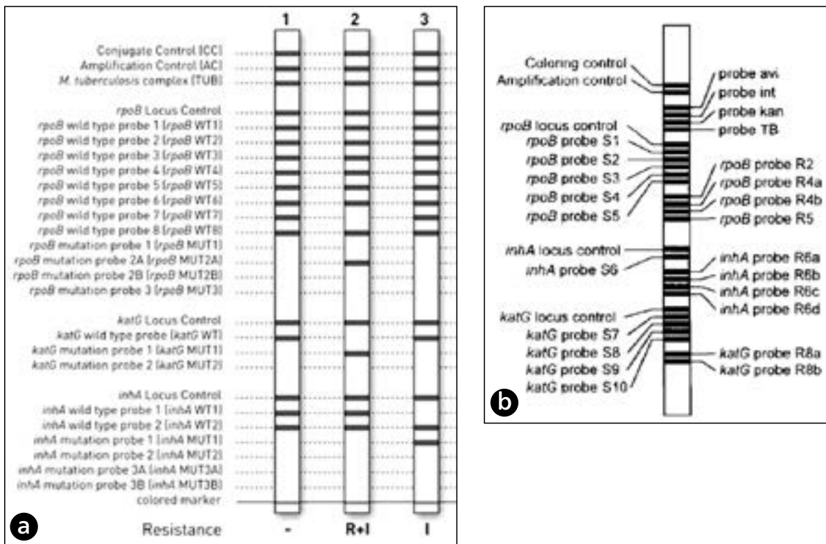
Fig. 2.3.5. Examples of different line probe assay strip readouts: (a) Hain GenoType MTBDRplus version 1 and version 2 (Hain Lifescience, Nehren, Germany) and (b) Nipro NTM+MDRTB Detection Kit 2 (Nipro, Tokyo, Japan)
