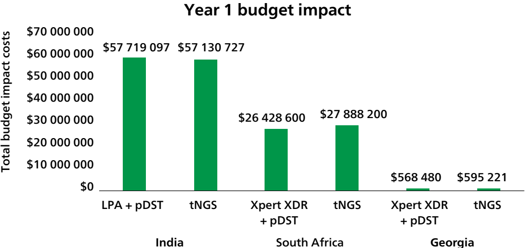
Fig. 2.3.11. Budget impact assessment results comparing current standard practice for DST to implementing targeted NGS for patients with RR-TB in India, South Africa and Georgia
