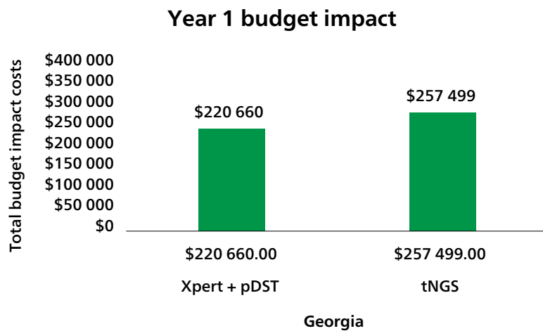
Fig. 2.3.10. Budget impact assessment results comparing current standard practice for DST with implementation of targeted NGS for all patients diagnosed with TB in Georgia
