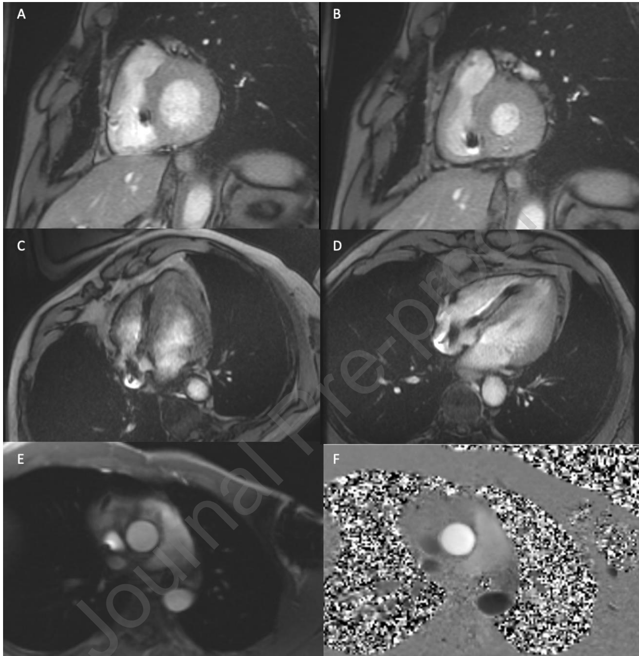
Figure 3. Exemplary CMR images in a patient with a left-sided CIED including short-axis GRE post-contrast images at end-diastole (A) and end-systole (B); 4-chamber GRE images pre-contrast (C) and post-contrast (D); and 2D phase contrast imaging at the ascending aorta (E, magnitude; and F, phase).
